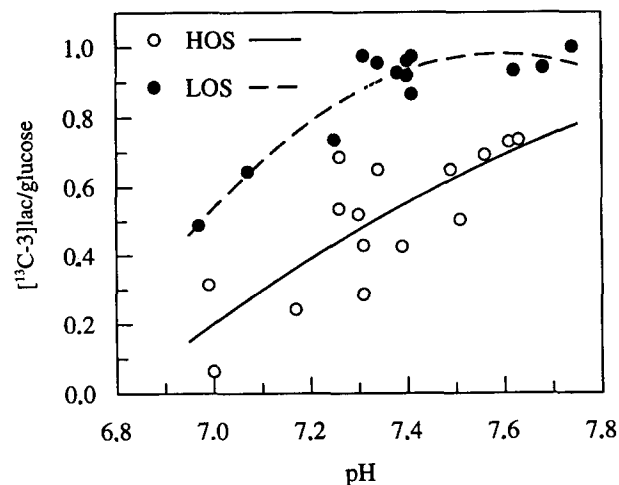
Fig. 3. Ratio between [^{13}\text{C-3}]\text{lactate} production and glucose consumption measured on HOS and LOS erythrocytes incubated with ^{14}\text{C} -1-labelled glucose as a function of pH (80 mM phosphate). Difference highly significant ( P < 0.0001 ).
